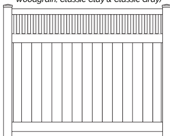
Z31* Closed Picket (Top Rail: T-Rail or 2x3 1/2)
