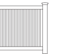
Z11* w/ 7/8 x 1-1/2" Picket or 1-1/2" sq 1-3/4" Spacing
